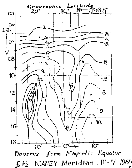
Fig. 2 — Synthetic plot for March equinox with f_oF_2 variation.
