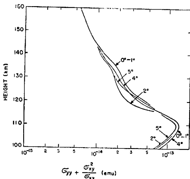
Fig. 4 — \sigma_{yy} + \sigma_{xy}^2/\sigma_{xx} versus height. Dip angle is shown on each curve.
