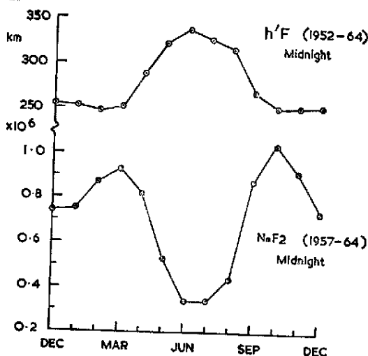
Fig. 6 — Variations throughout the year of midnight h'F and mid-night NmF2.
