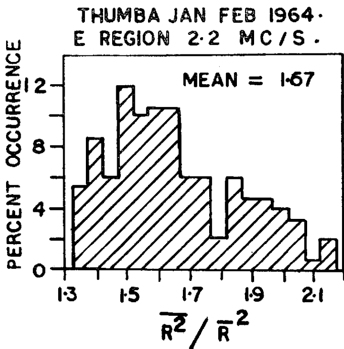
Fig. 2 — Histogram of the values of the ratio of mean squared amplitude and square of mean amplitude of Es reflection over Thumba.
