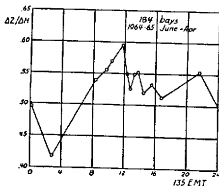
Fig. 4 — Ratio of vertical to horizontal amplitude of bays at Koror, for Jun. 1964 to Apr. 1965.
