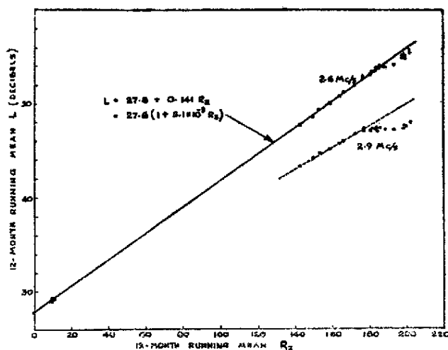
Fig. 2. VARIATION OF NOON ABSORPTION WITH SUNSPOT NUMBER
