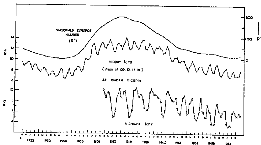
Fig. 1 — Variations of monthly median midday foF2 (crosses) and midnight foF2 (circles) at Ibadan and of smoothed sunspot number, R^* , (continuous line) from 1952 to 1964.
