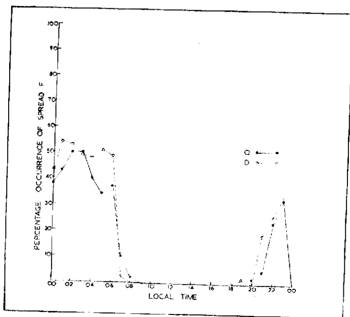
Fig. 1 — Percentage of occurrence of spread-F versus local time for quiet and disturbed days for the whole year.
