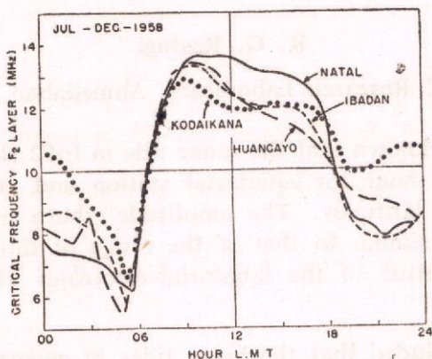
Fig. 2 — Mean daily variation foF2 at the equatorial stations, showing abnormal variation at Natal.
