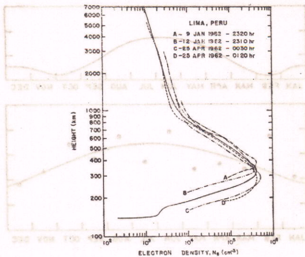
Fig. 3 — Electron density profiles at the magnetic equator, obtained around midnight using the incoherent scatter technique. Curves A, B, C and D, after Bowles et al.; full line curve, smoothed average. Average value of absorption corresponding to these profiles is 0.1 db. This value of absorption can be obtained by calculation using the average profile and Nicolet's expression for collision frequency (between electrons and positive ions) when the electron temperature is taken as 550°K.
