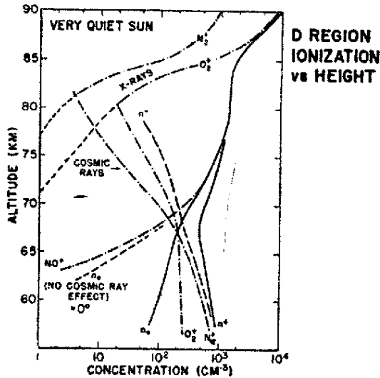
Fig. 3 — The distribution of positive and negative ions and electrons as predicted by Nicolet and Aikin (4)
