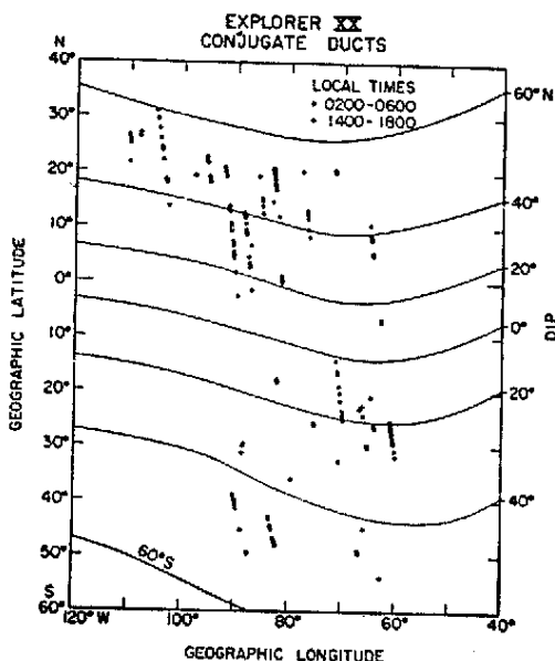
Fig. 2 — The locations of conjugate ducts observed during September 1964. Curves of constant dip are also shown.
