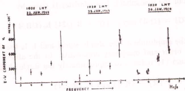
Fig. 2 — East-west component of V_c in m/s for the same observations of Fig. 1. Note the frequency dependence of V_c .
