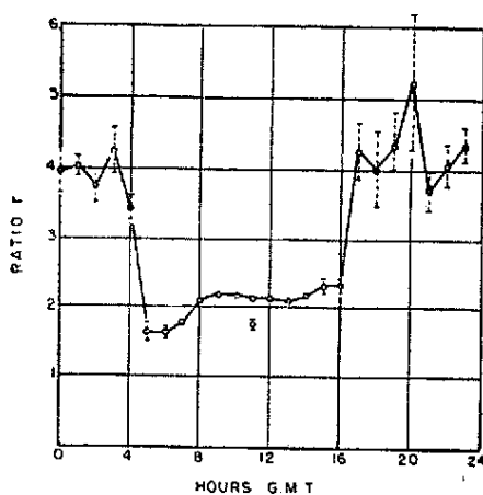
Fig. 15 — Diurnal variation of amplitude ratio H/Z for irregular fluctuations in Nigeria (from Onwumechilli, 1959).
