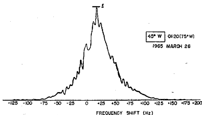
Fig. 2 — Power spectrum obtained during nighttime in the same way as for Fig. 1.
