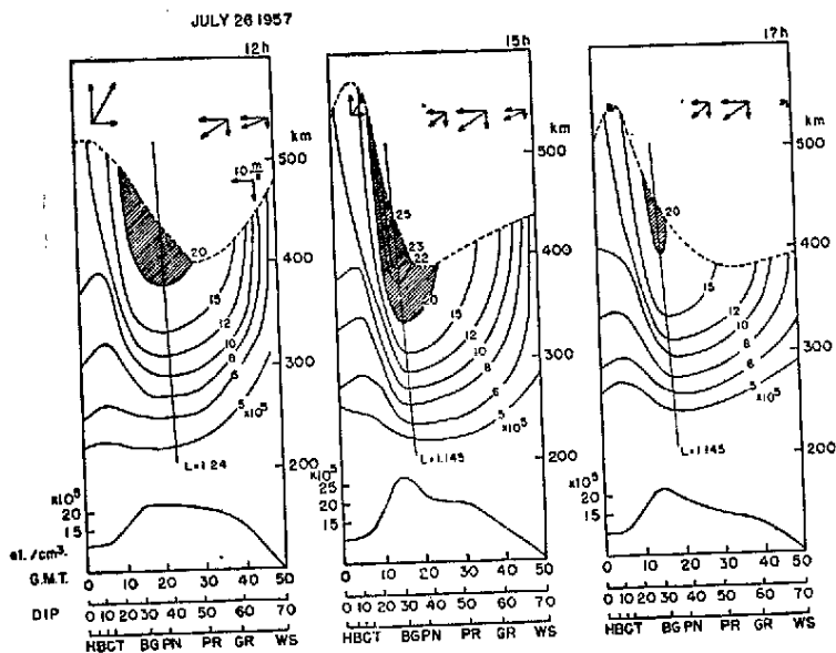
Fig. 2 — Sequential time variation of the vertical profile of electron density in the 350° geomagnetic meridian plane. The lower curves show the maximum electron density distribution, the line contours of the F region density, the dotted lines the height of the maximum electron density, the thin lines the geomagnetic line of force and the arrows the velocity vector of the ionization drift.
