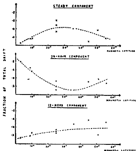
Fig 1. Variation with latitude of the relative importance of the harmonic components of F-region drifts.
