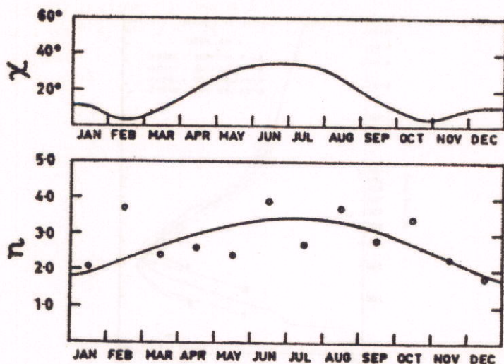
Fig. 4 — Bottom figure: the values of the exponent n in the equation A = K (foF2)^n for the different months at Huancayo. Top figure: Seasonal variation of midday values of solar zenith angle \chi at Huancayo.
