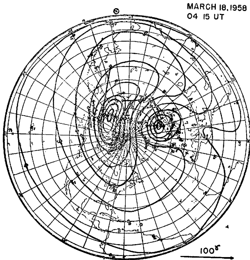
Fig. 3 — Equivalent current system for the case shown in Fig. 2.
