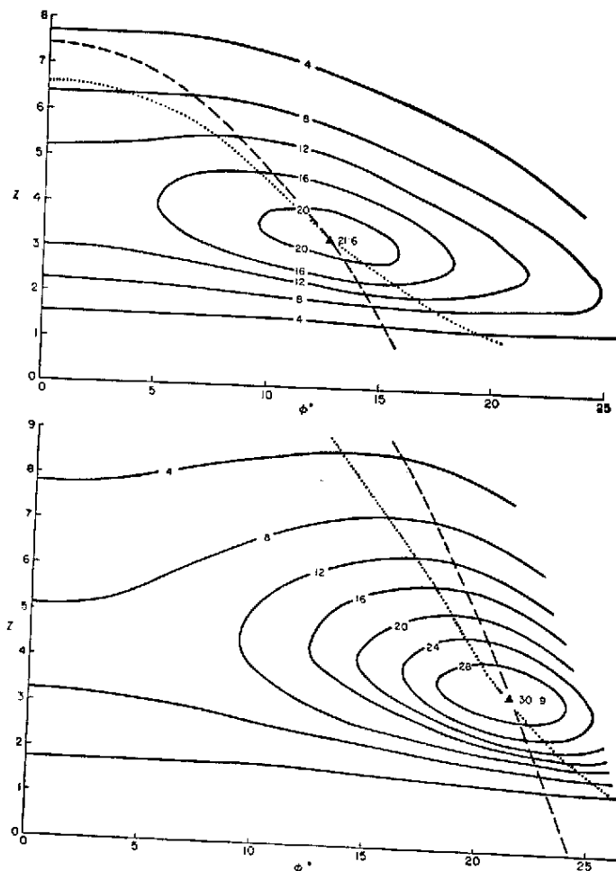
Fig. 1 — Contours of electron density (in units of 10^5 \text{ cm}^{-3} ) as a function of latitude and height. The height is measured in units of 1 scale height of the ionizable gas (82 km) above a reference level of 180 km. The vertical drift speed at the reference level is 4.1 \text{ m sec}^{-1} for the top figure and 20.5 \text{ m sec}^{-1} for the bottom one.
