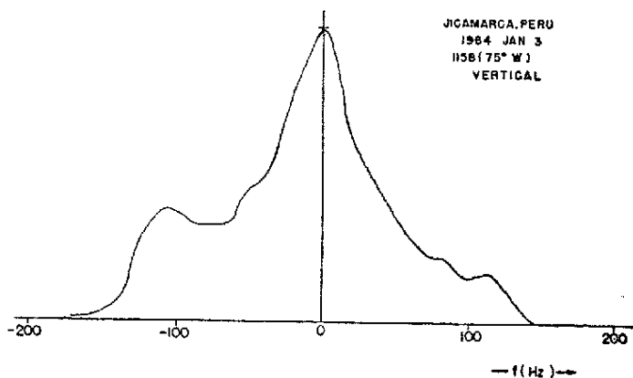
Fig. 3 — Same for a well-developed electrojet.
