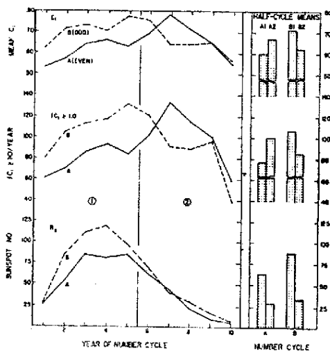
Fig. 2 — A comparison of magnetic activity, number of disturbed days and sunspot number from one cycle to another. The change in level of terrestrial magnetic activity for each half of each cycle is shown by the bar graphs at the right and indicates the nature of the sunspot-magnetism cycle in this aspect.
