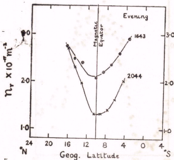
Fig. 3 — VARIATION WITH LATITUDE OF TOTAL ELECTRON CONTENT n_T
