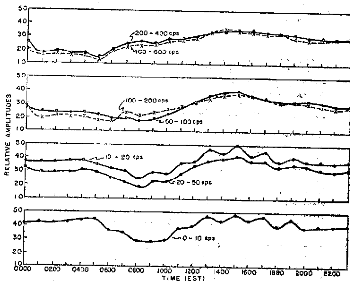
FIG. 2 DIURNAL VARIATION IN SIGNAL AMPLITUDES IN FREQUENCY RANGES: 0-10 cps, 10-20 cps, 20-50 cps, 50-100 cps, 100-200 cps, 200-400 cps, AND 400-600 cps FOR OCT. 7-16, 1964 AT HUANCAYO, PERU
