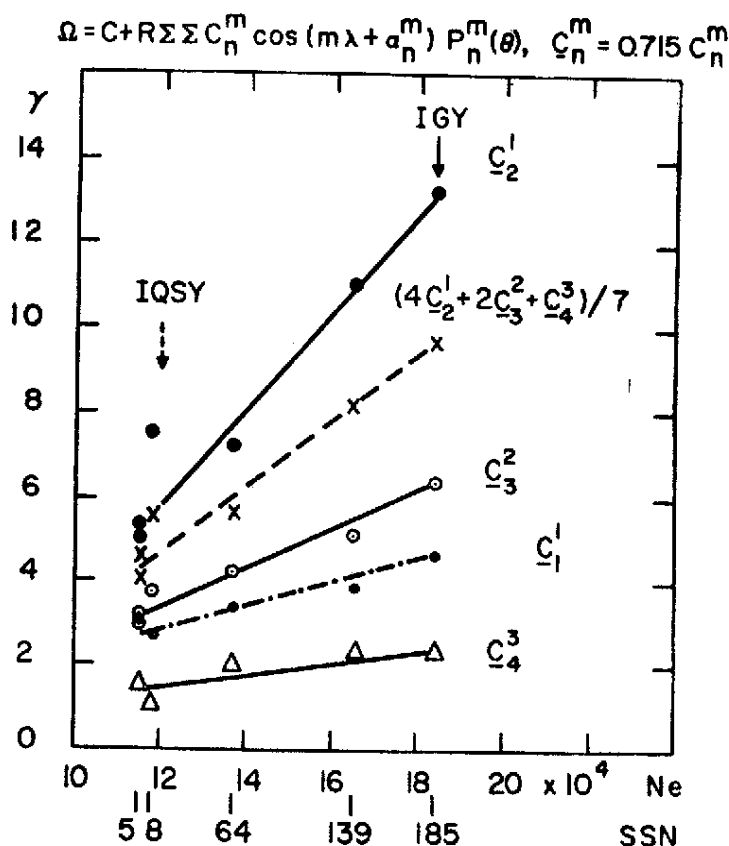
Fig. 1 — Main terms of external origin plotted with respect to sunspot number and electron density in the E region. Also plotted is a weight mean (dashed line).
