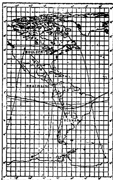
Fig. 1 — The VLF transmission paths: NBA-Boulder and NBA-Tucuman. The basic map showing approximate geomagnetic meridians and the position of the geomagnetic equator at ground level (thin line) and 100-km altitude (thick line) was taken from Dudziak et al (2) .
