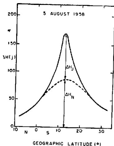
Fig. 2 — Illustrating the method used for determining the degree of enhancement of the world wide Sq current at the dip equator.
