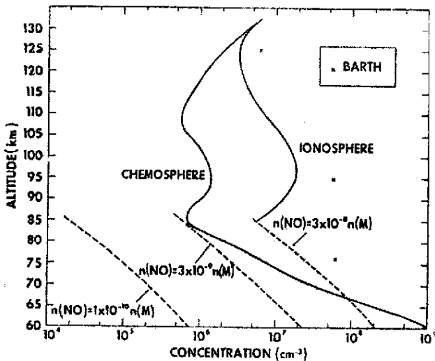
Fig. 5 — The nitric oxide distribution in the 60 to 130 km altitude range
