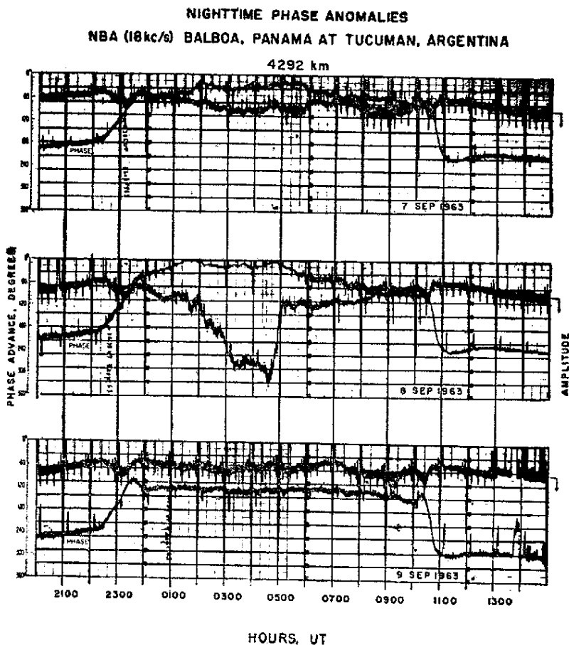
Fig. 5 — Photographs of the actual phase and amplitude recordings made at Tucuman on the 7, 8, and 9 September 1963. On the left the phase scale is one complete cycle at 18 kHz in degrees of phase advance. On the right the relative field strength trace is identified and the direction of an amplitude increase is indicated.
