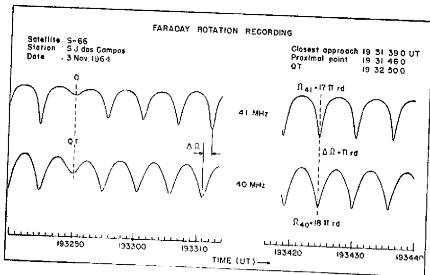
Fig. 1 — Recording of the Faraday rotation of polarization in the 40 and 41 MHz beacons of S-66, showing the quasi transverse (QT) propagation region ( \Omega = 0 ) and a case with \Omega_{40} = 18 \Delta\Omega .
