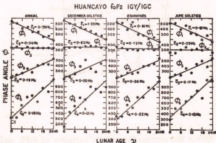
Fig. 6 — Shows similar diagrams for foF2 during IGY-IGC. The phase of second harmonic is again independent of the lunar age indicating that the lunar perturbations are predominantly tidal in nature.
