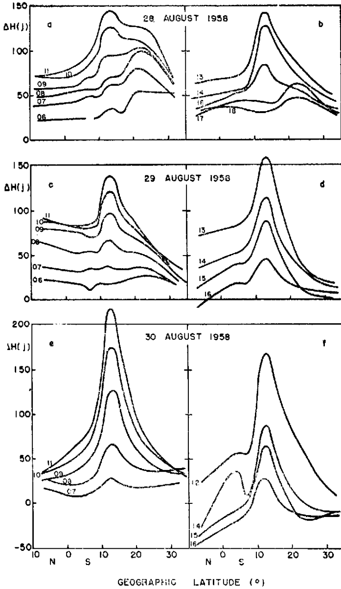
Fig. 1 (a-f) — The \Delta H latitudinal variations in South America for 3 successive Quiet Days during the IGY.
