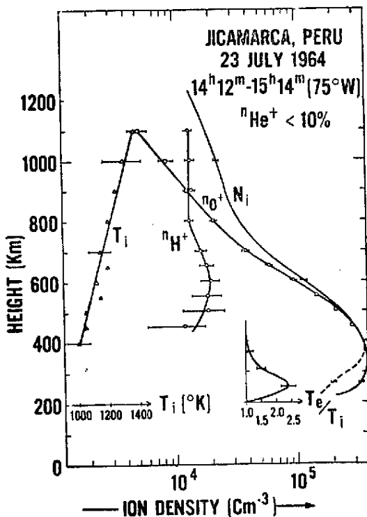
Fig. 2 — Daytime ion composition results inferred by Bowles et al. using incoherent scatter at Jicamarca, which is at the geomagnetic equator.
