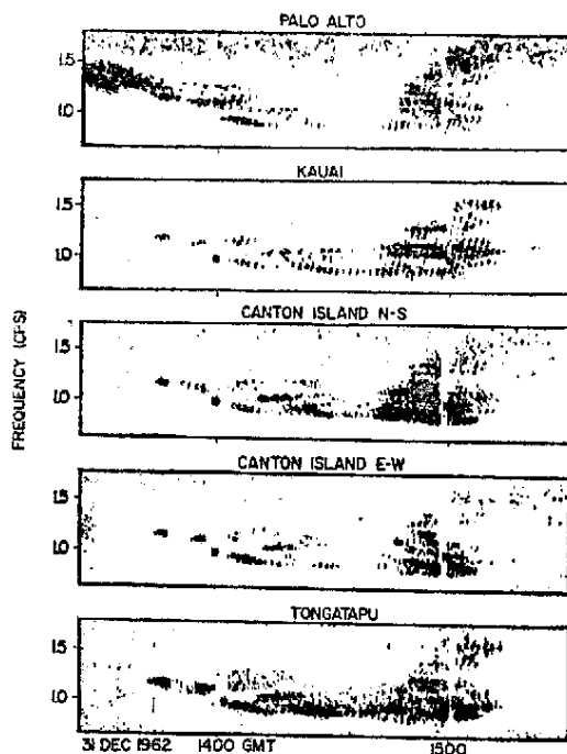
Fig. 2b — Pc-1 pulsations spectra at Kauai, Canton, and Tongatapu (from Tepley, 1964).
