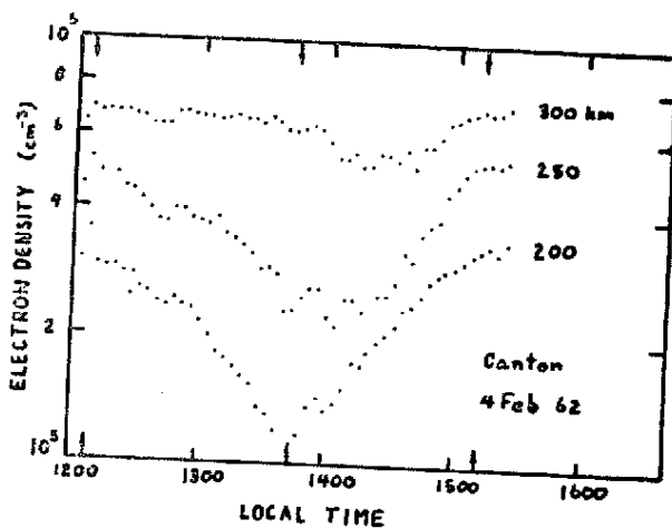
Fig. 2 — Electron density at fixed heights plotted versus time. The eclipse times are indicated by the arrows.
