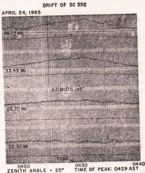
Fig. 4 — N_o scintillations have been noted in this extended source of 16' (3C392). This is the smallest source which failed to produce scintillations in the study.
