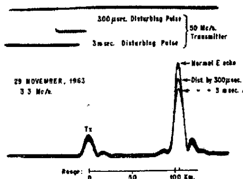
Fig. 2 — An illustration of how the cross modulation changes as the disturbing pulse is lengthened.
