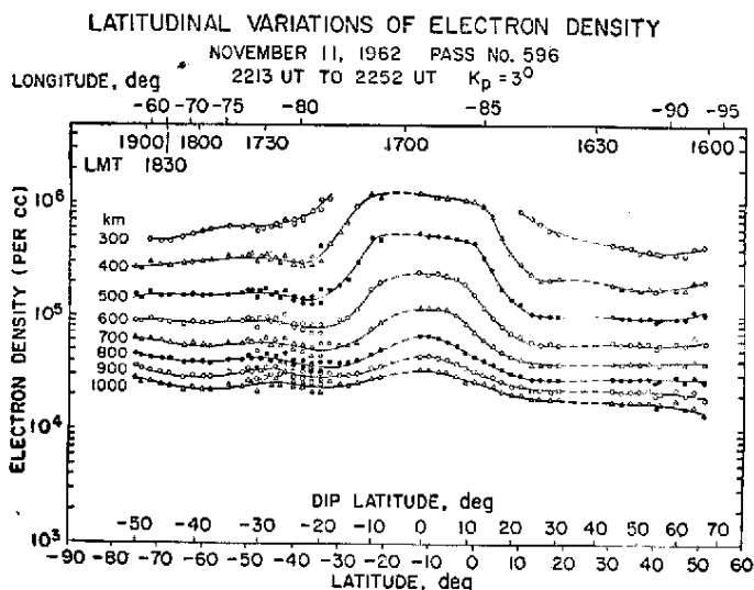
Fig. 1 — The latitudinal variation of electron density for pass 596 of the Alouette satellite.
