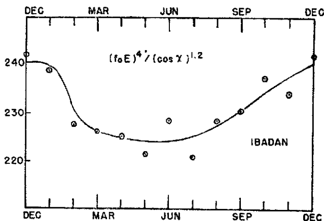
Fig. 3 — Annual variation of the quantity (foE)^4 / (\cos \chi)^{1.2} , proportional approximately to the rate of electron production q .
