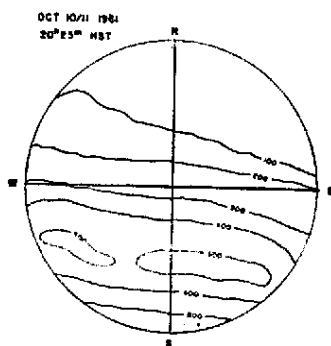
Fig. 5 — Isophote map showing existence of a 6300 Å aurora from observations at Haleakala (Maui, Hawaii).
