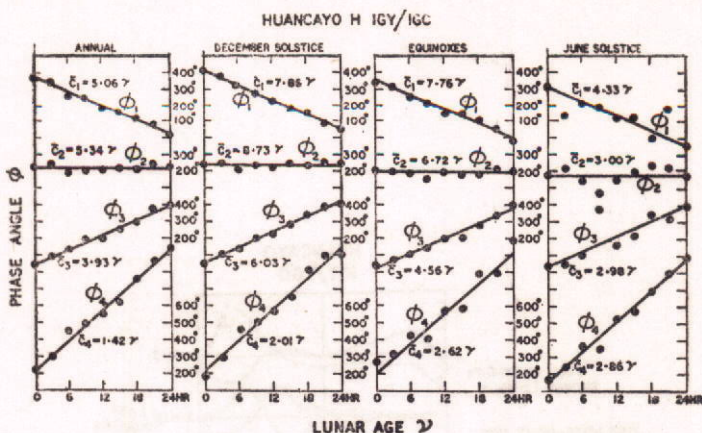
Fig. 5 — Shows the first, second, third and fourth harmonic components of lunar daily variations in H at Huancayo during different lunar age in different seasons of the year. The curves indicate that the Chapman's phase law is very closely followed by these variations. The phase of second harmonic is independent of lunar age.
