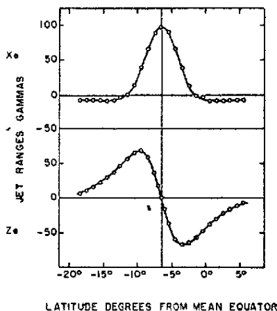
Fig. 5 — Showing how the field model fits electrojet field derived from observations (points) in Peru at equinox 1957.
