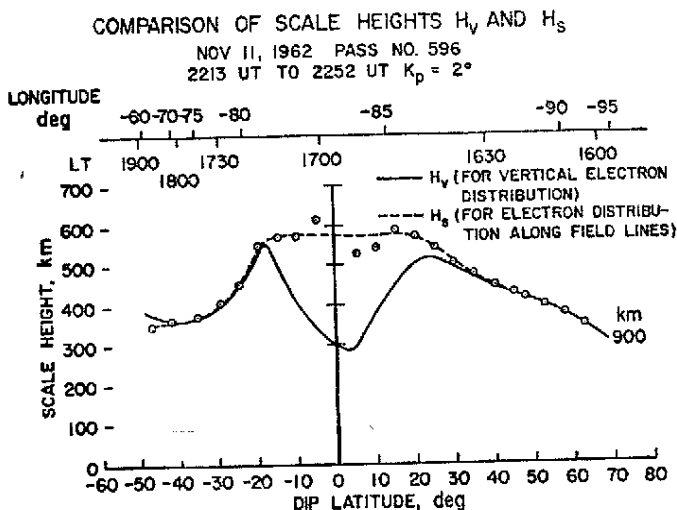
Fig. 5 — The vertical scale height, H_v , for 900 km on pass 596 (see Figs. 1 and 2) has been converted into a field aligned scale height, H_s . The large minimum in H_v near the dip equator is removed and H_s may be used to deduce the ratio of effective temperature T_0 mean ionic mass in the usual way.
