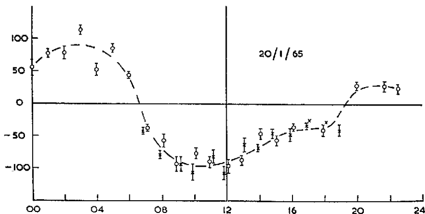
Fig. 3 — Diurnal variation of eastward component of drift velocity at Ibadan on a single day. Circles are for the F region and crosses for the E region. The error bars have been computed assuming the irregularities to be accurately field aligned.
