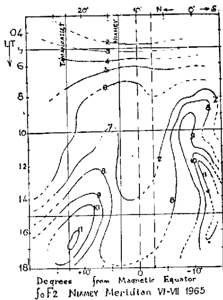
Fig. 3 — Idem for solstice of the previous plot.
