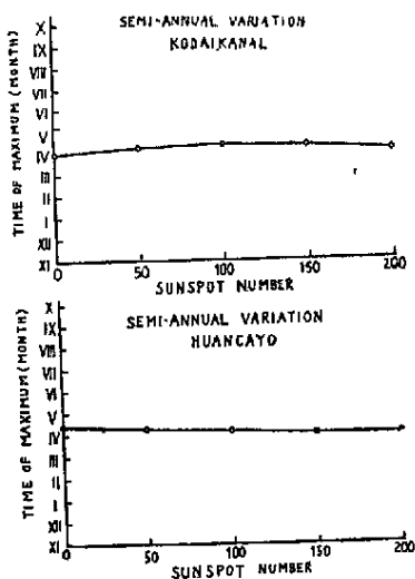
Fig. 6 — Times of maximum of the semi-annual variations for Kodai-kanal and Huancayo as functions of sunspot number.
