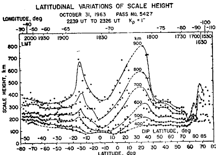
Fig. 4 — The latitudinal variation of scale height, H_s , for pass 5427.
