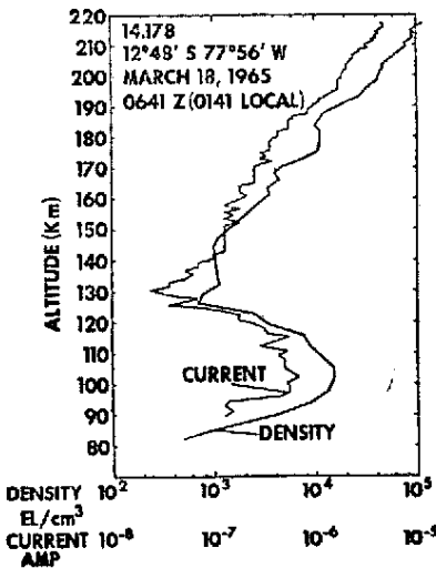
Fig. 3 — Electron density and Langmuir probe current as a function of altitude observed on 14.178 at 0141 LMT.
