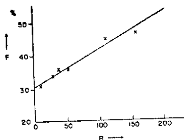
Fig. 1 (a) — Variation of spread-F occurrence frequency, F , with sunspot number.
