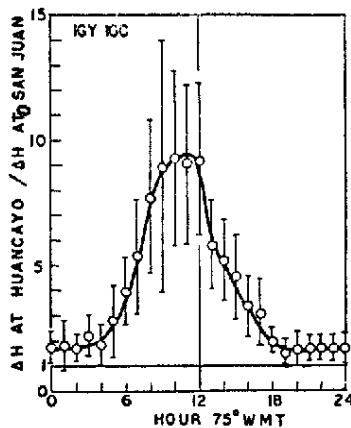
Fig. 3 — Daily variation of the ratio of deviations in H at Huancayo and at San Juan.
