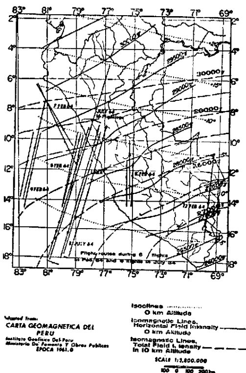
Fig. 1 — Chart of the geomagnetic field intensity and dip in Peru after Casaverde and Giesecke showing the aircraft flight paths.
