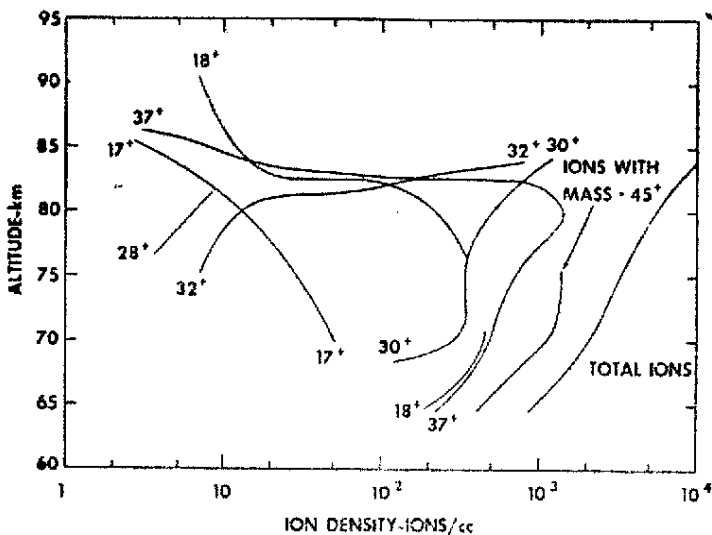
Fig. 4 — Ion composition in the D region as measured by Narcisi and Bailey (6)
