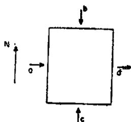
Figure 2: a + b + c \neq d , showing unbalance of currents in ionospheric element.
