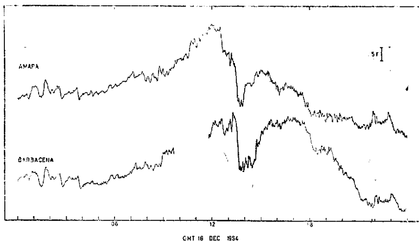
Fig. 2 — Total magnetic field intensity records for one day at the conjugate stations. There is a data gap in the Barbacena record.
