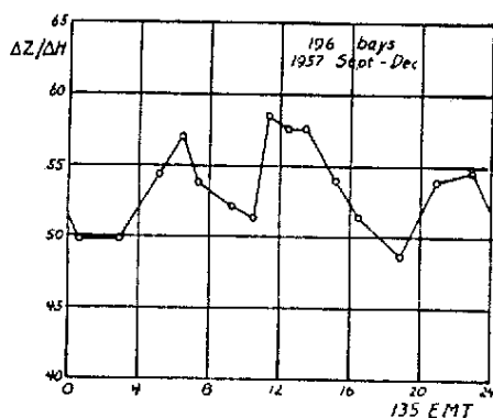
Fig. 3 — Ratio of vertical to horizontal amplitude of bays at Koror, for Sept.-Dec. 1957.
