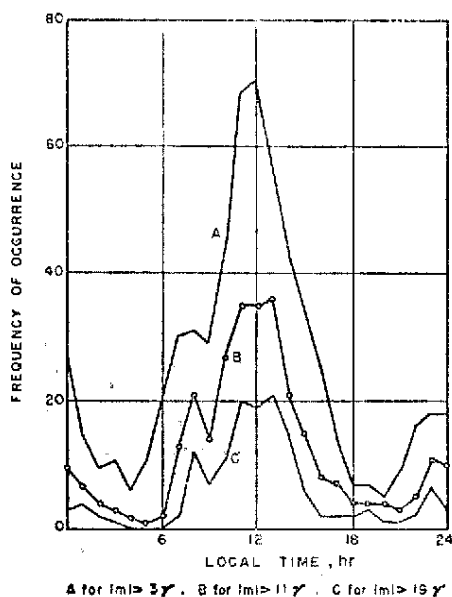
Fig. 14 — Occurrence frequency of irregular fluctuations in Nigeria (from Onwumechilli, 1960).
