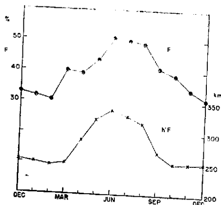
Fig. 2 — Annual variations (a) of spread-F occurrence frequency, F , throughout the night and (b) of midnight h'F .
