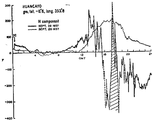
Fig. 2 — The Huancayo H records for 1957 September 28 (a quiet day) and 29 (including part of a great magnetic storm); on the 28th the record shows Sq, and the beginning of Sq is shown also on the 29th. Then the great storm began, with first a DCF increase and then a much larger decrease (DR). On this, between 1600 and 1900 GMT, is superposed the effect of an intense eastward return current of a westward auroral electrojet; despite the big H reduction caused by the DR current near the height of the main phase, the DP return current brings H above the normal maximum value around local noon. At this time the DP current much enhances the normal eastward Sq current along the electrojet. (Akasofu and Chapman, 1963; Fig. 4).
