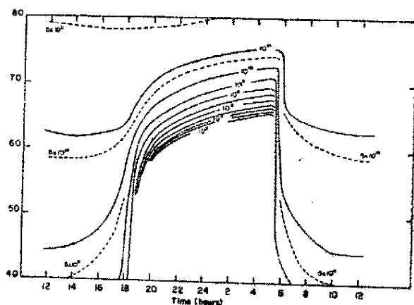
Fig. 1 — Photochemically produced diurnal variation of O at the Equator for an oxygen atmosphere. The ordinate represents height in km and the curves of constant densities are in \text{cm}^{-3} .
