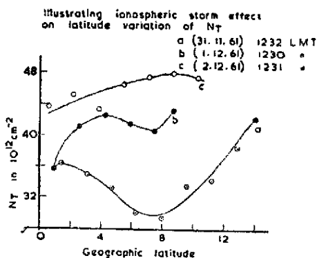
Fig. 4 — A daytime increase of the total columnar ionization during a storm is shown to be a regular feature. In the great majority of cases, h_m F_2 is not altered by a storm. The increase in ionization density occurs mostly in the topside ionosphere.
