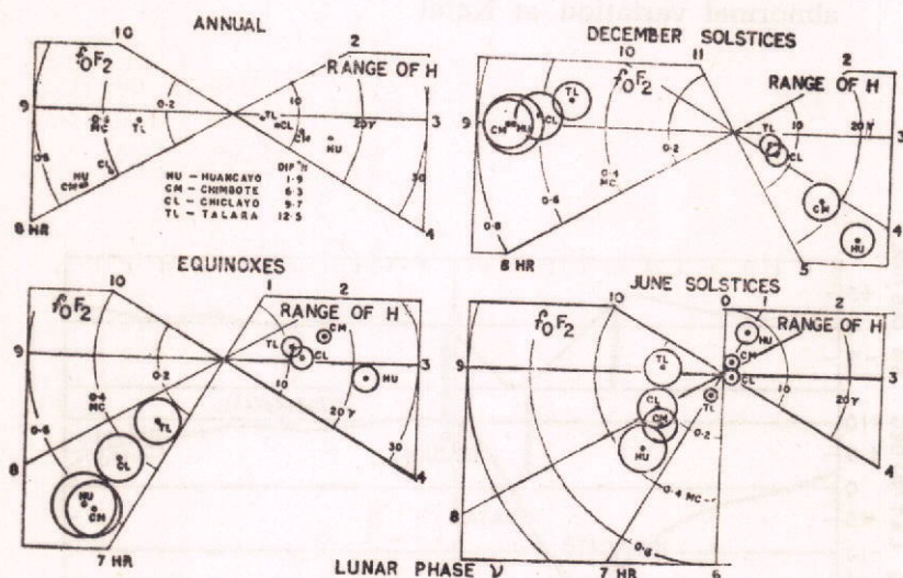
Fig. 1 — Shows the harmonic dials of the lunar tides in noon f_oF_2 and daily range in H at Peruvian stations during different seasons of IGY-IGC. The amplitude of tides in both f_oF_2 or range H increase progressively with decreasing latitude. The phase of lunar tide changes slightly with season, but the difference in phase of tides in f_oF_2 , and range H remains almost constant.
