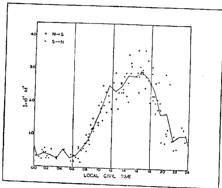
Fig 1 — Gives the hourly medians of total electron content I for the period October 1964 to January 1965 inclusive; the points show north- and south-going passes separately but all are included in the medians. The values were obtained from the fading rate at the zenith together with a constant value of 3000 gammas per degree for the latitude derivative dM/d\lambda , horizontal gradients are neglected but the records do not, in general, indicate large horizontal gradients in daytime.
