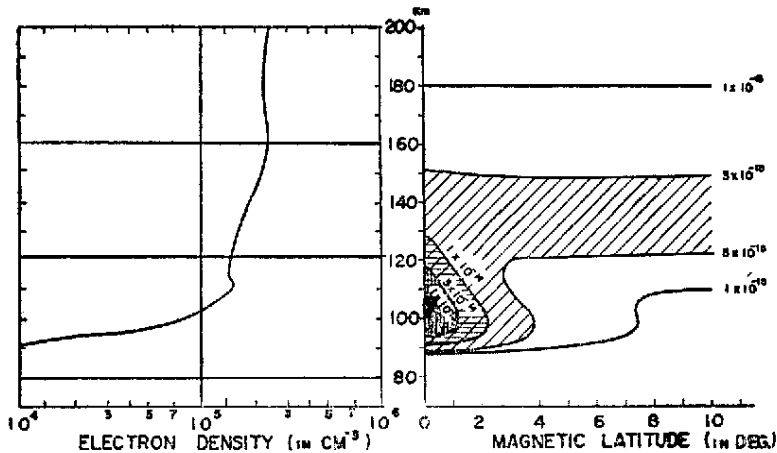
Fig. 3 — Profile of the conductive sheet (right) deduced from a model of the ionosphere during daytime (left). Conductivity is indicated in emu.
