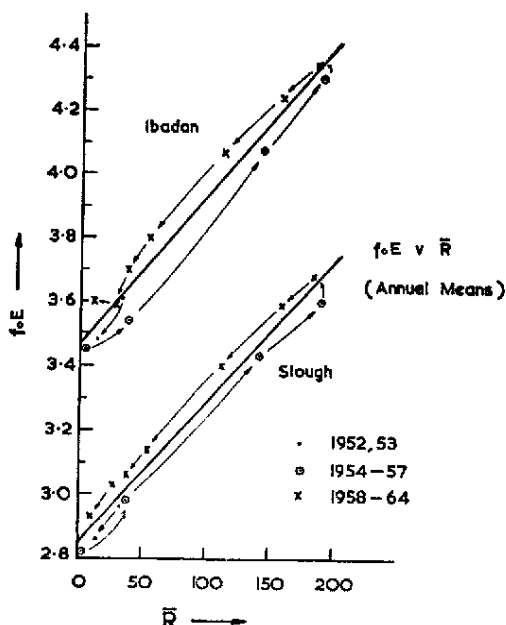
Fig. 1 — Variations of annual mean foE at noon with annual mean sunspot number at Ibadan and at Slough. Circles are for the rising phase and crosses for the falling phase of the cycle, and arrows indicate the direction of change in successive years.
