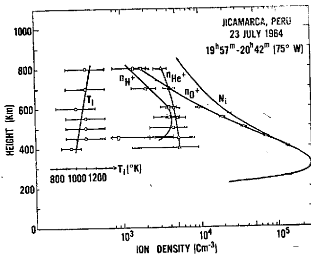
Fig. 3 — Nighttime ion composition results inferred by Bowles et al. using incoherent scatter at Jicamarca.
