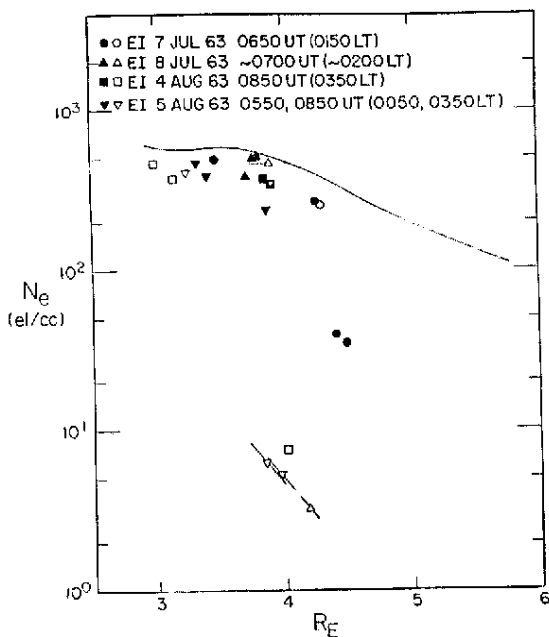
Fig. 2 — Four different equatorial profiles corresponding to post-midnight hours when the magnetic activity is moderate ( K_p in the range 2 to 4). Note the sharpness and repeatability of the "knee" both in position and density. The continuous line represents the profile of Fig. 1 and is shown as a reference.
