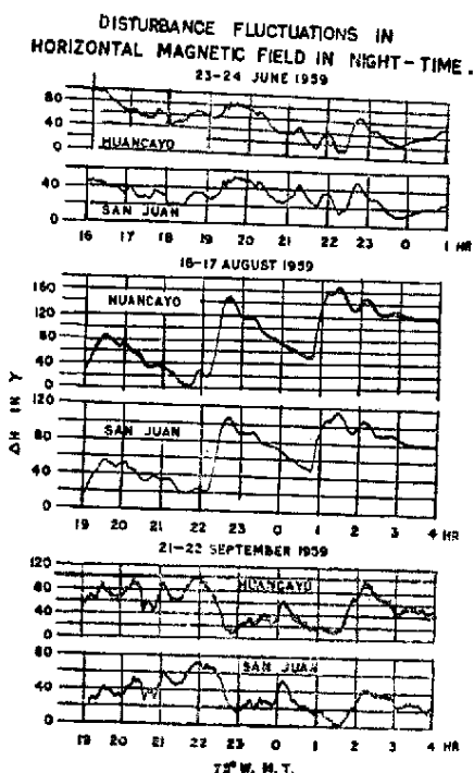
Fig. 2 — Tracings of H magnetograms at Huancayo and San Juan during nighttime disturbances.
