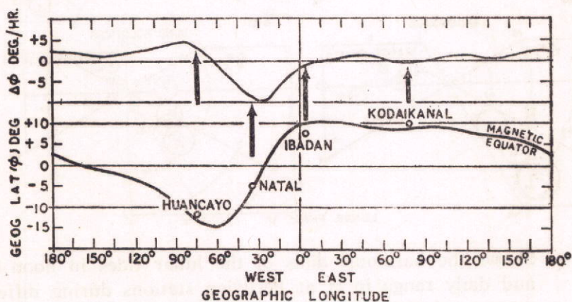
Fig. 3 — Position of the magnetic equator at different longitude and the deviation in the position of the magnetic equator for one hour change in the universal time.
