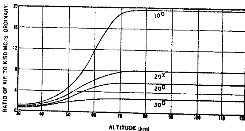
Fig. 1 — The ratios of the absorption coefficients in the lower ionosphere to the absorption coefficient for 50 MHz, for several different frequencies and modes. ( 20^0 denotes the ordinary mode on 20 MHz; 20^X is the extraordinary mode). At altitudes greater than about 70 km, the ratio is given by the ratio of the squares of the frequencies. At altitudes below about 30 km, there is no frequency dependence. In the region 30 < Z < 70 km, the absorption coefficients are not simply related, and electron profile determinations may be done here.
