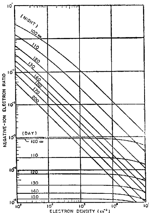
Fig. 2 — The ratio ( \lambda ) of negative ion density to electron density as a function of electron density at various heights.
