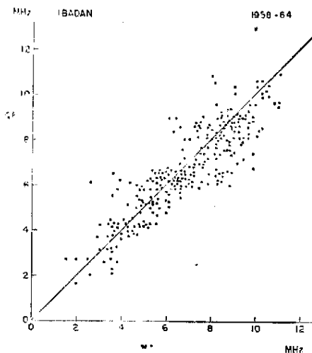
Fig. 3 — A mass plot of top frequency of spread-F (ordinary wave, denoted by symbol QF) against corresponding interpolated values (denoted by "INT").
