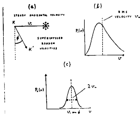
Fig 2. The ionospheric model. (a) The directions of the velocities. (b) The distribution of random velocities. (c) The resolved velocity distribution along KK' .
