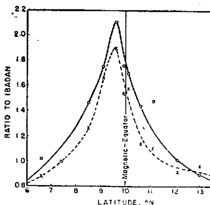
Fig. 17 — Equatorial enhancement of daily amplitude ratio of irregular fluctuations (from Onwumechilli and Ogbuchi, 1962).
