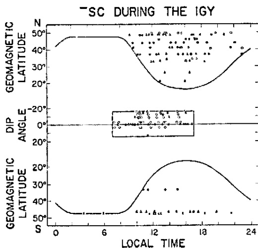
Fig. 1 — Occurrences of -SC at worldwide IGY stations between the geomagnetic latitudes 50°N and 50°S are shown against the local time of occurrence and the latitude of the station (the dip angles in the magnetic equatorial zone). The solid circles, triangles, crosses, and open circles indicate the following four longitudinal zones: Europe and Africa (gm 50°E-140°E), Asia and Australia (gm 140°E-320°E); and Northwest and South America (gm 320°E-50°E), (Matsushita, 1964).
