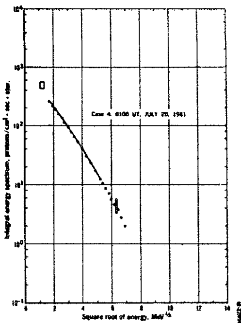
Fig. 2 — A solar cosmic ray energy spectrum determined from multifrequency riometer data taken during the July 1961 solar cosmic ray events. The dots connected by a line are points calculated from the multifrequency riometer; the two rectangles are derived from the Injun 1 satellite data. The good agreement is indicative of the accuracy which can be obtained with the multifrequency riometer technique.
