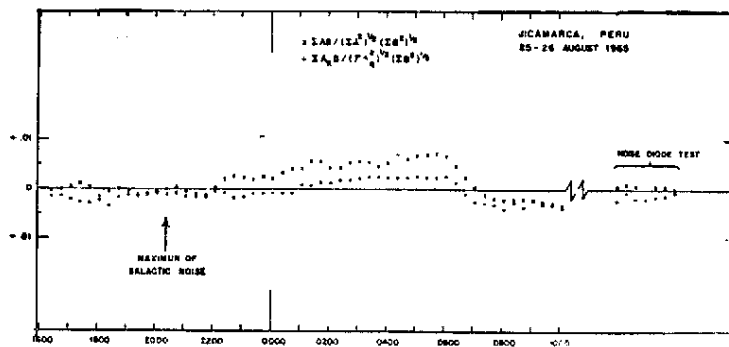
Fig. 2 — Synchrotron radiation observations. The maximum value of the galactic noise at 2000 hrs. was about 45,000°K, whereas the minimum value at 0600 hrs. was about 5000°K. The measurements near 2000 hrs. show that \gamma , the voltage cross-talk ratio, was of order 10^{-3} or less. The observations near 0600 hrs. give a value of synchrotron noise power of about 35 K. Note the Faraday rotation occurring after sunrise as the ionosphere builds up.
