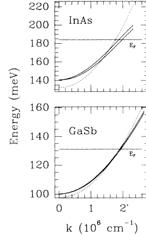
FIG. 2. Spin-orbit (Rashba) split lowest subbands with nonparabolicity in InAs- and GaSb-based heterojunctions, both with n_s=6.0\times 10^{11} cm -2 . The Fermi energy and the parabolic approximation (dashed lines) are also shown. The zero of energy corresponds, in each case, to the bottom of the bulk conduction band.
