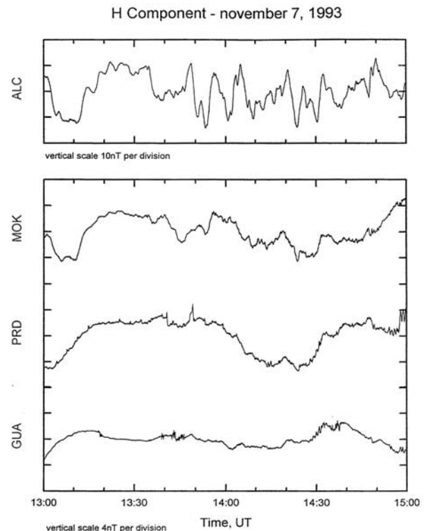
Figure 11. H component of ALC, MOK, PRD, and GUA ground magnetograms from 1300 to 1500 UT on 7 November 1993. See Table 1 for station names.
