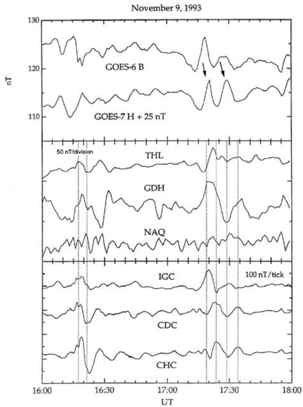
Figure 2. (top to bottom) GOES 6 and 7 geosynchronous magnetic field observations, the H component of Greenland ground magnetograms at THL, GDH, and NAQ, and the X component of Magnetometer Array for Cusp and Cleft Studies (MACCS) array stations IGC, CDC, and CHC from 1600 to 1800 UT on 9 November 1993. Vertical dashed lines after 1710 UT identify the times when Zesta et al. [1999] identified four TCVs in the ground observations. Vertical dashed lines prior to 1630 UT identify large-amplitude perturbations at CDC that cannot be interpreted as TCVs. See Table 1 for station names.
