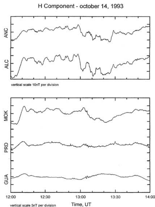
Figure 7. H component of ANC, ALC, MOK, PRD, and GUA ground magnetograms from 1200 to 1400 UT on 14 October 1993. See Table 1 for station names.
