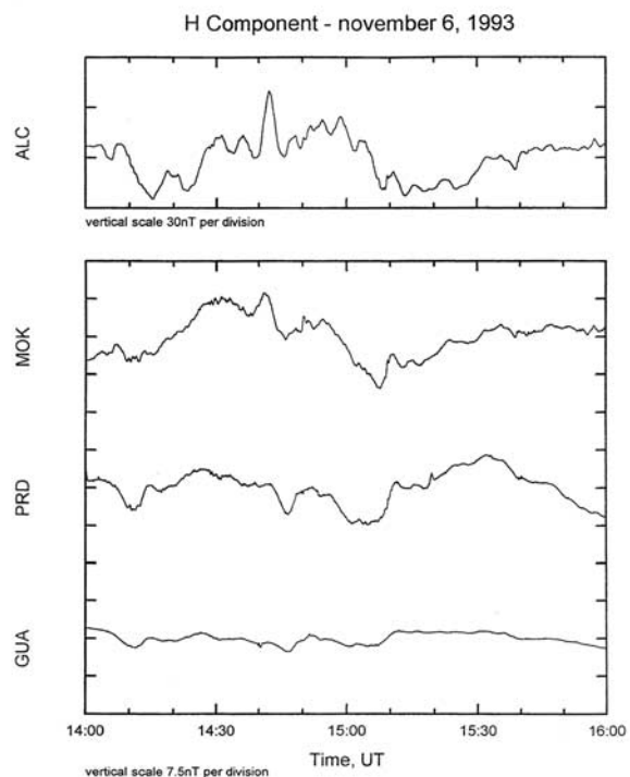
Figure 9. H component of ALC, MOK, PRD, and GUA ground magnetograms from 1400 to 1600 UT on 6 November 1993. See Table 1 for station names.
