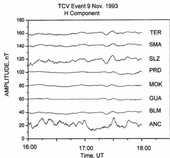
Figure 3. H component of ANC, GUA, MOK, PRD, BLM, SLZ, SMA, and TER ground magnetograms from 1600 to 1800 UT on 9 November 1993. See Table 1 for station names.
