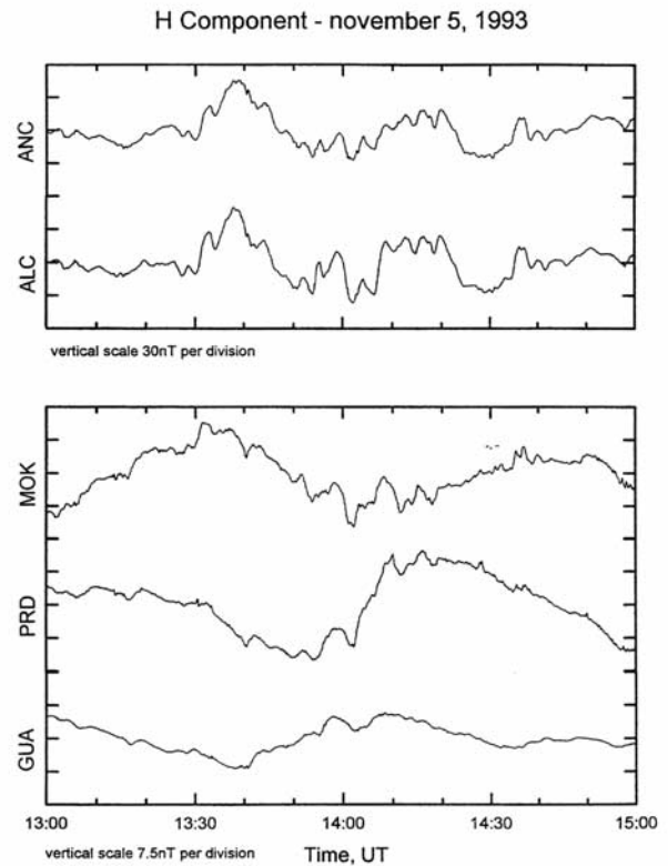
Figure 13. H component of ALC, MOK, PRD, and GUA ground magnetograms from 1300 to 1500 UT on 5 November 1993. See Table 1 for station names.
