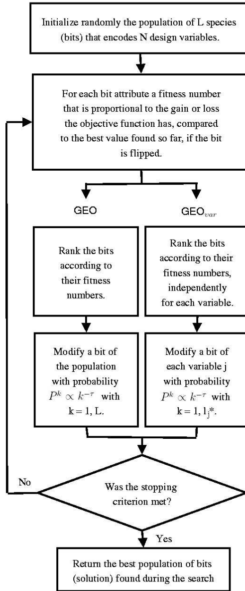
Figure 4. Flowchart of GEO and GEO var , where l_j^* is the number of bits of each variable j , with j = 1, N (from [Sousa et al. 2003])
