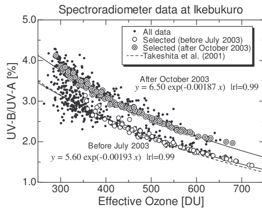
Figure 3: The UV ratio of the spectroradiometer at Ikebukuro versus effective ozone evaluated from Tsukuba ozone data. Data points are separated into two parts. Dashed line means the result of Takeshita et al. (2001).
