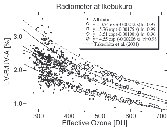
Figure 4: UV ratio of the radiometers at Ikebukuro versus effective ozone. The scatter of data is larger and four fitting results are obtained depending on the combinations of radiometers.
