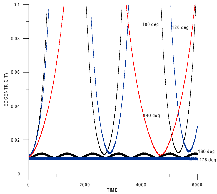
Figure. 4- Evolution of the eccentricity.
