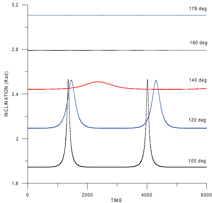
Figure. 3- Evolution of the inclination.
