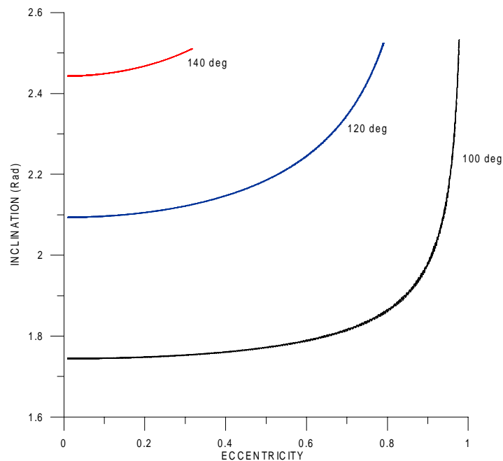
Figure. 8- Evolution of inclination vs eccentricity.
