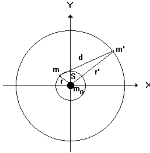
Fig. 1. Illustration of the third body perturbation.
