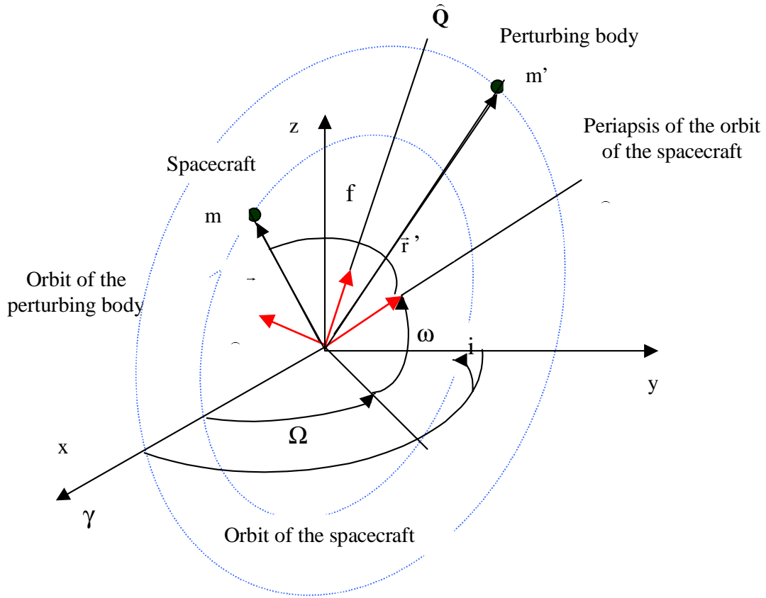
Fig. 2. The orthogonal set \hat{P} , \hat{Q} , \hat{R} and the coordinate system in the orbital plane.
