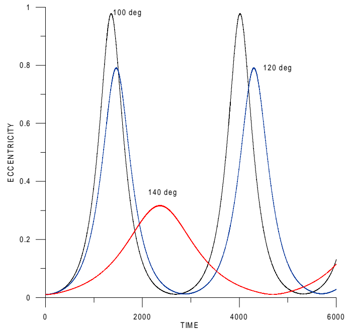
Figure. 5- Evolution of the eccentricity.
