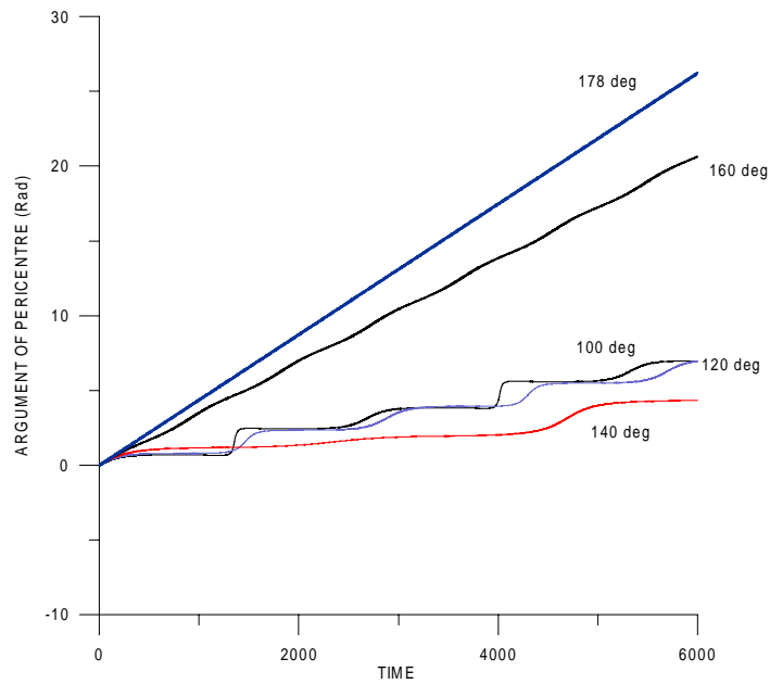
Figure. 6- Evolution of the argument of pericenter.
