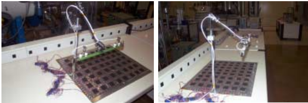
Figure 1: Experimental apparatus.
