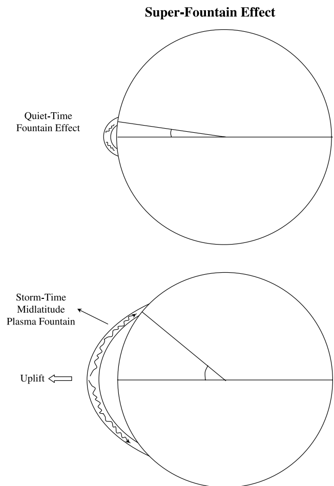
Figure 13. A schematic of a “superfountain effect,” which may explain plasma enhancements at midlatitudes. The quiet time fountain effect is illustrated in the top panel. Uplift of equatorial plasma is followed by flow along magnetic field lines, leading to enhanced densities at \sim \pm 15^\circ MLAT. In cases of extremely strong uplift during intense storm-time eastward electric fields, the spread of plasma will reach midlatitudes.
